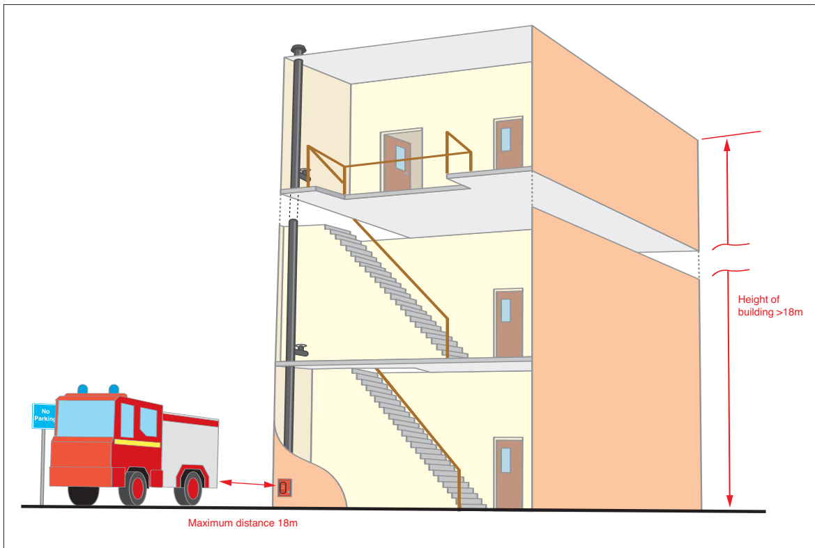
Figure 20: Rising main
